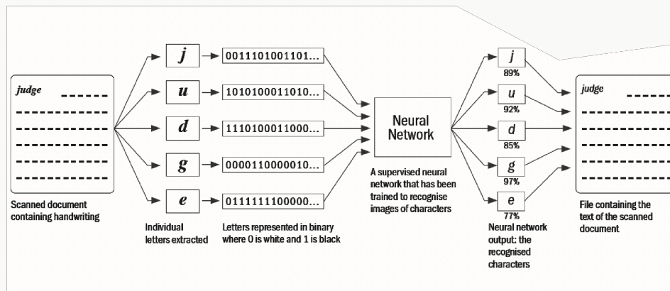
Figure 4: Using a neural network to identify handwriting
